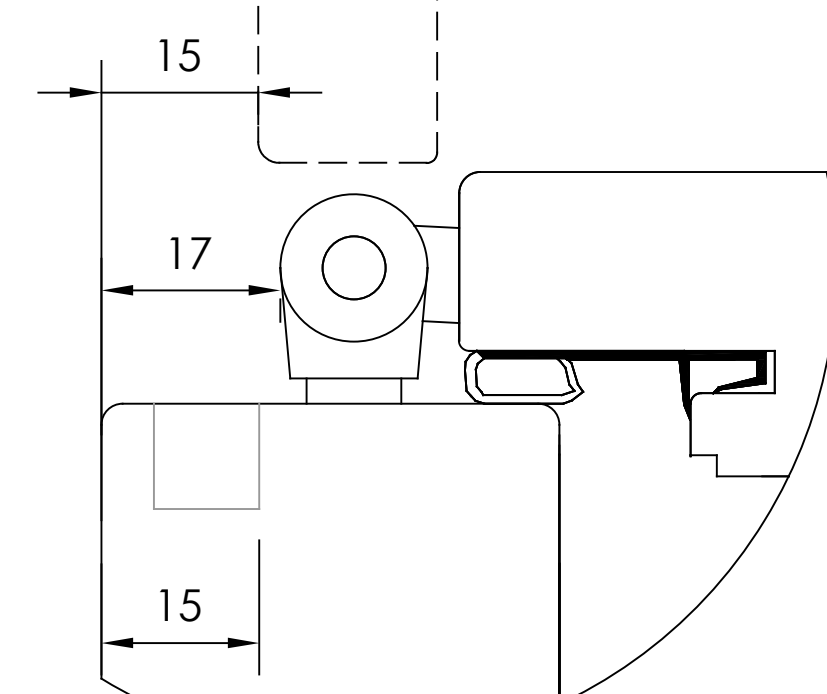
- Exterior hinges
